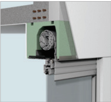
PLASTER (MONOLITHIC)
